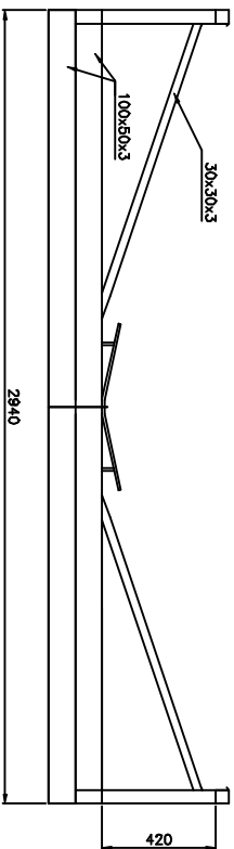
AFT VIEW
