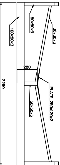
AFT VIEW
